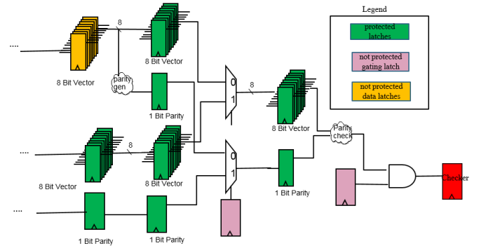
Figure 3. A parity protected structure.
