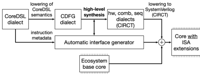
Figure 3: High-level synthesis flow for ISA extensions.
