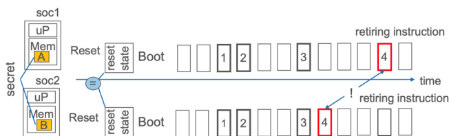
Figure 5: UPEC on unrolled SoC model.
