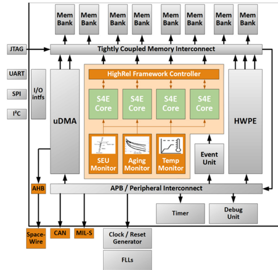
Figure 10: Architecture of HiRel demonstrator.
