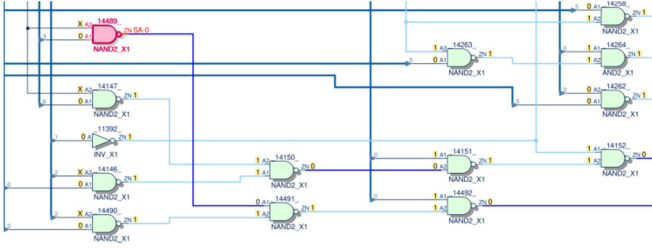
Figure 7: Visualization of a test pattern for a stuck-at-fault in DarkRISC-V. The affected gate and the propagated fault effect are shown using different colours.
