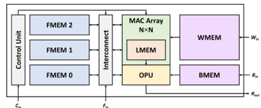
Figure 9: Overview of the UltraTrail architecture.
