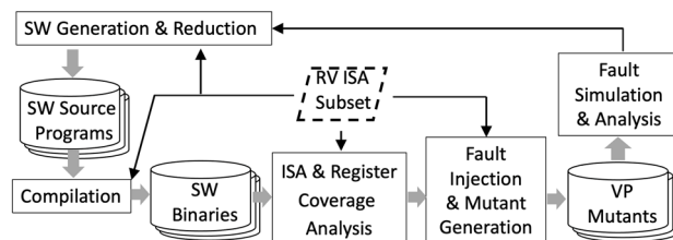
Figure 6: Scalable framework for fault coverage and simulation.
