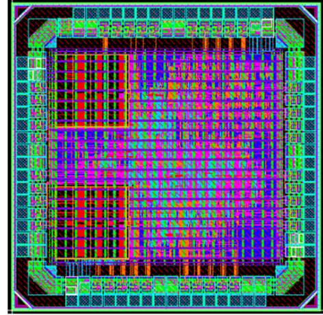
Figure 8: Ecosystem demonstrator Version 1 layout.
